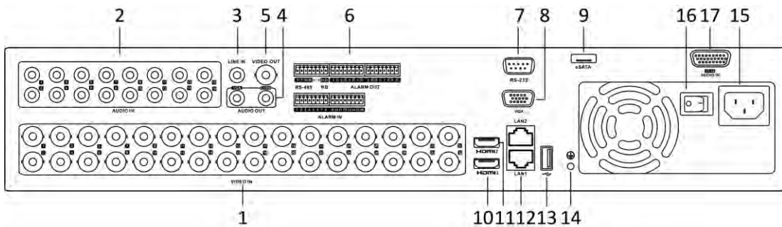
Figure 1-18 Rear Panel of DS-8100HQHI/HUHI-K8 (with 32-ch Video Inputs)
