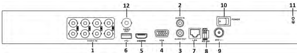
Figure 1-12 Rear Panel of DS-7200HQHI-K/P
