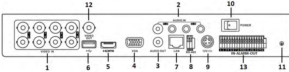
Figure 1-9 Rear Panel of DS-7200HUHI-K
