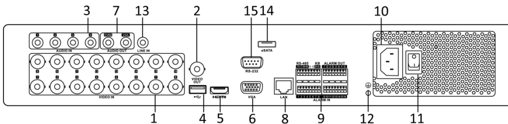
Figure 1-13 Rear Panel of DS-7300HQHI-K (with 16 Video Inputs)
