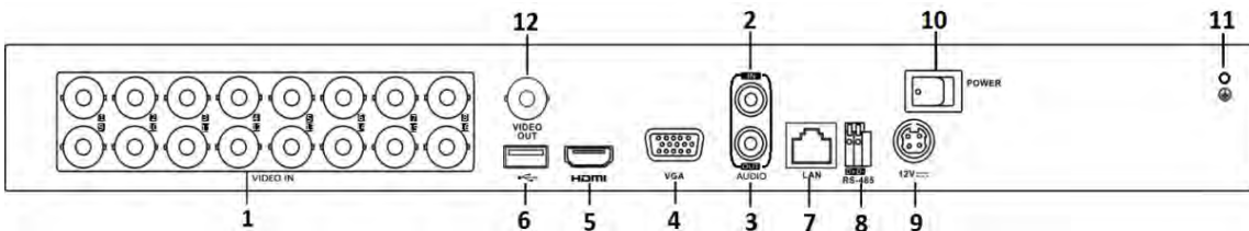
Figure 1-11 Rear Panel of DS-7200HQHI-K
