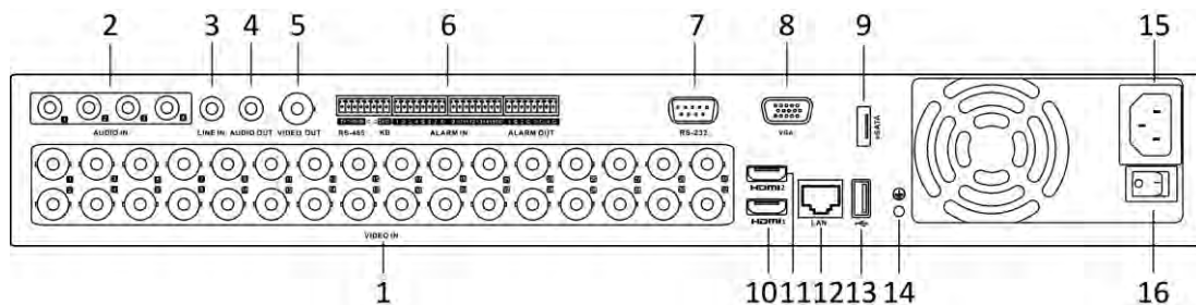
Figure 1-16 Rear Panel of DS-7300HQHI-K4 (with 32-ch Video Inputs)
