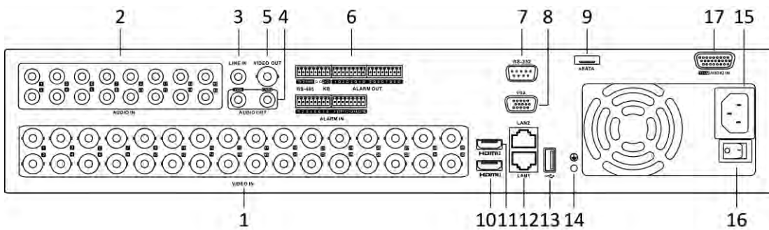
Figure 1-19 Rear Panel of DS-9000HUHI-K8 (with 32-ch Video Inputs)
