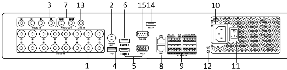
Figure 1-14 Rear Panel of DS-7300HUHI-K4 (with 16 Video Inputs)
