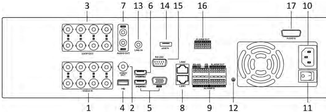
Figure 1-15 Rear Panel of DS-9000HUHI-K8 (with 8 Video Inputs)
