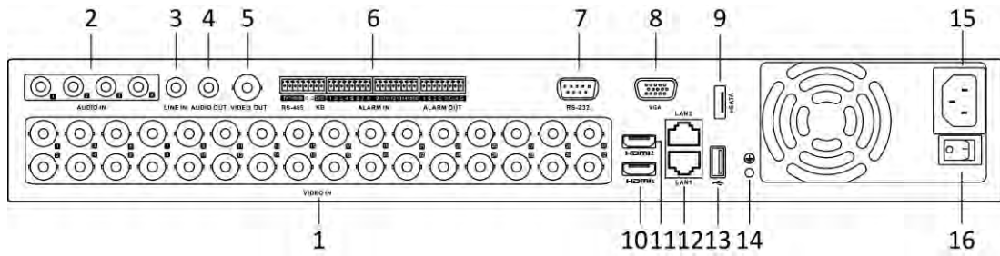
Figure 1-17 Rear Panel of DS-7300HUHI-K4 (with 32-ch Video Inputs)
