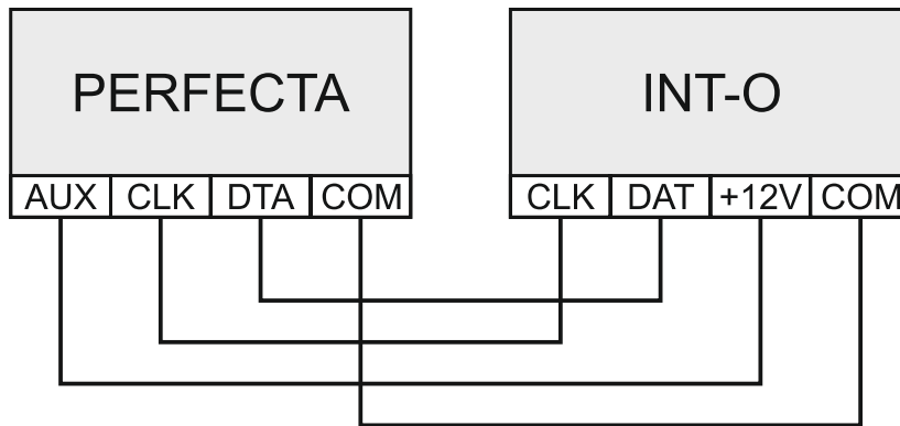
Fig. 7. Connecting the INT-O expander to the control panel.
