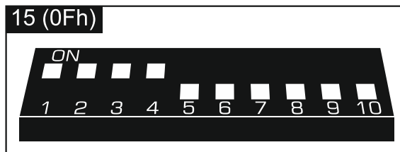
Fig. 8. Setting DIP-switches in the INT-O expander.
