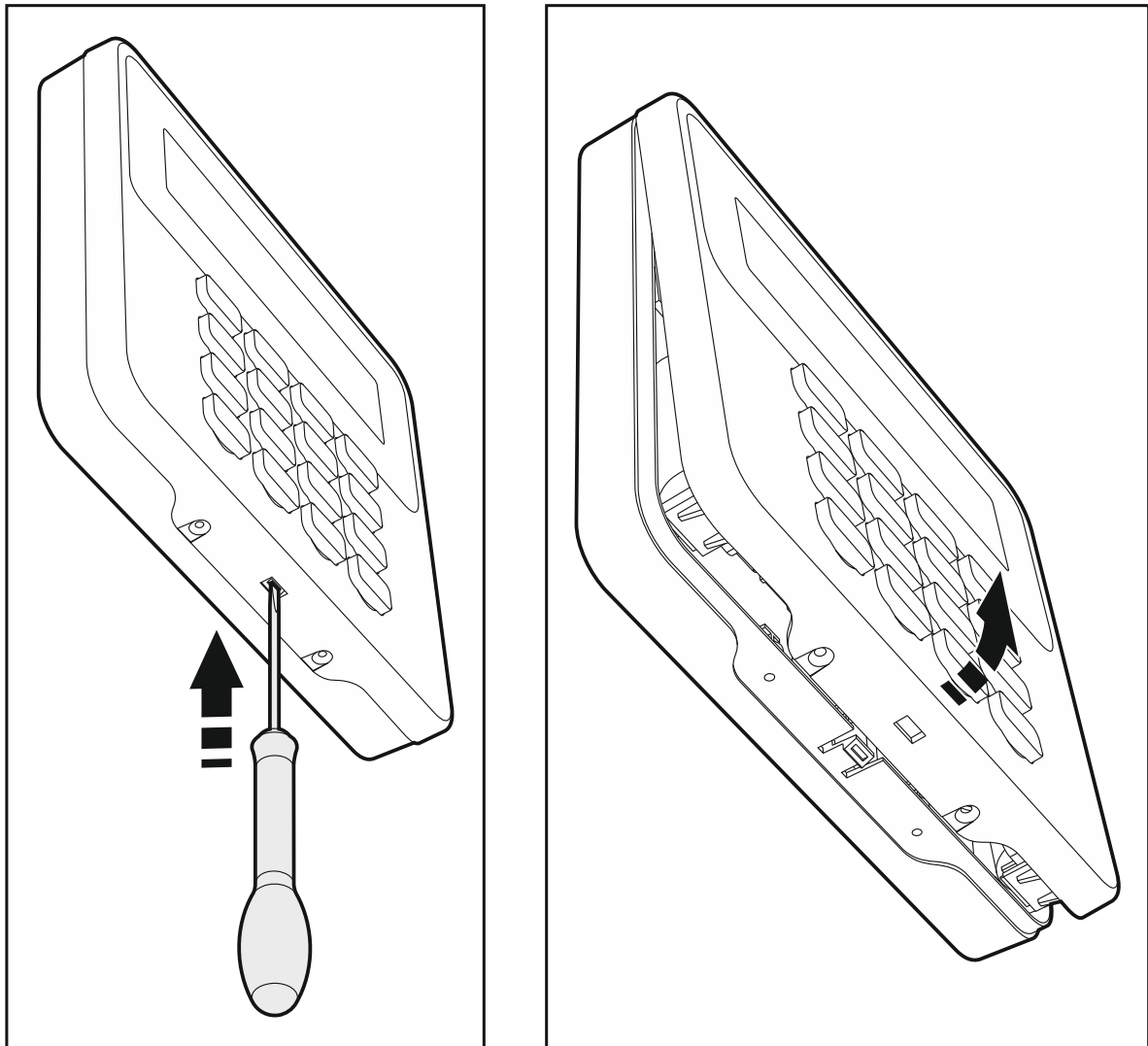
Fig. 3. Opening the keypad enclosure.
